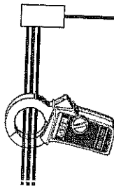
Fig.4 Earth Leakage Current Measurements
