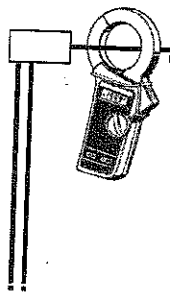
Fig.4 Earth Leakage Current Measurements
